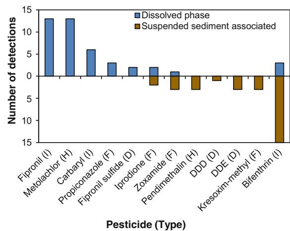
Fig. 3 Comparison of dissolved and suspended sediment associated pesticides in stormwater. Includes compounds detected in >1 sample ( n = 20 samples). Pesticide types: F , fungicide; H , herbicide; I , insecticide; D , pesticide degradate
